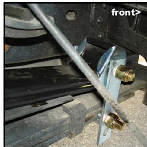
front> Front & Rear ~ mount spring with eye bolt threads out
