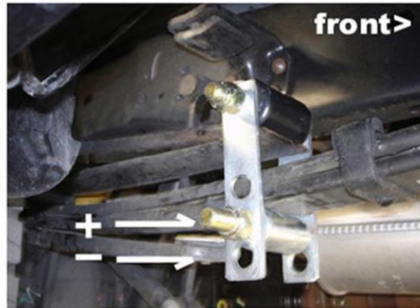
Place PSP11 on top of spring plate flat side up facing, with groove toward the front
