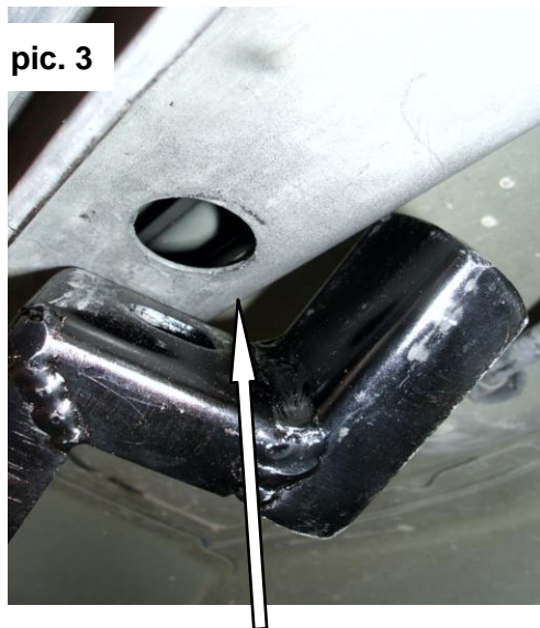
Hole / 3/8 " bolt plate
