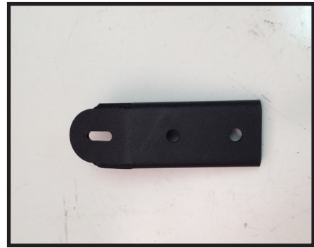
Part # 35130-07 / Qty. 2 Rear sway bar relocation bracket
