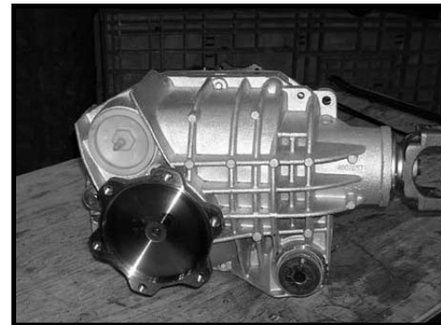
nose cut off of the front differential
